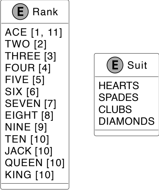
Suit and Rank Enums
