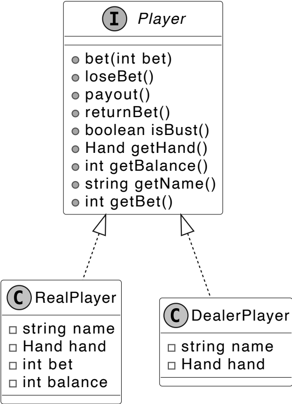
Player interface with concrete classes
