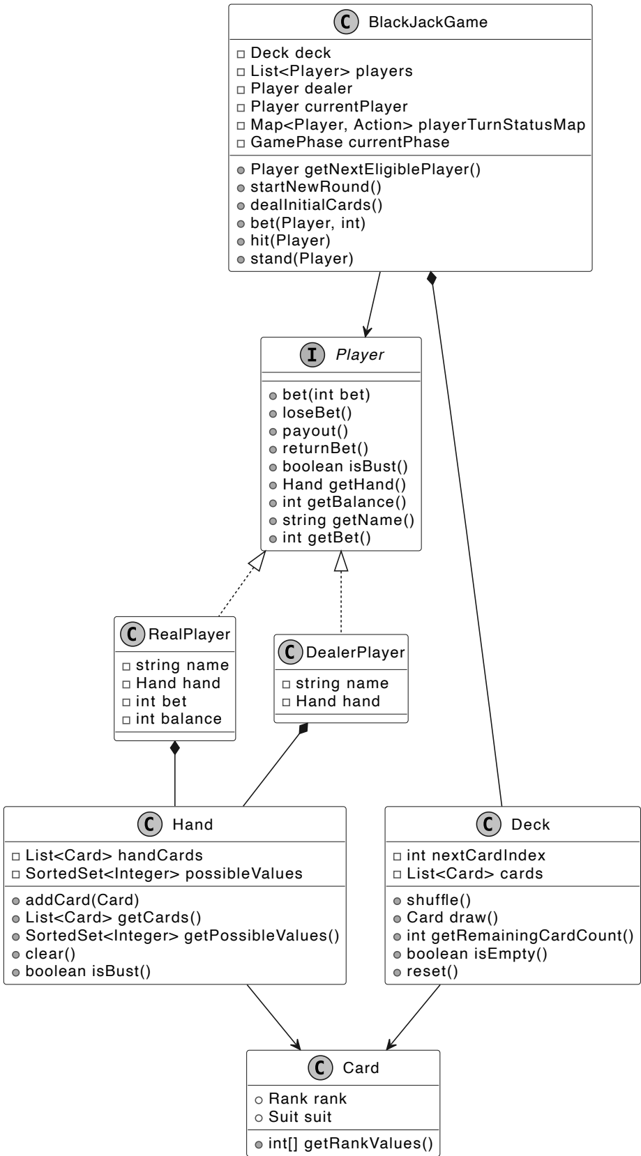
Class Diagram of Blackjack
