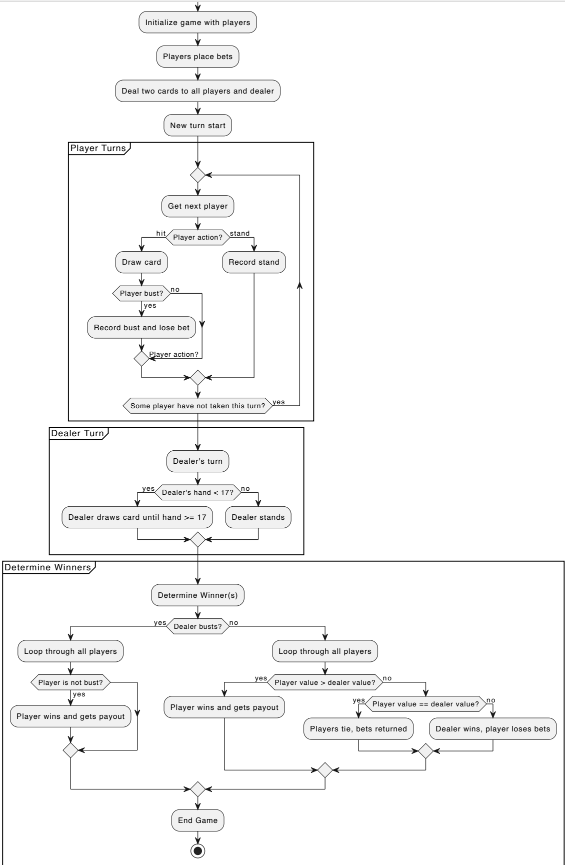
Activity Diagram of Blackjack Game
